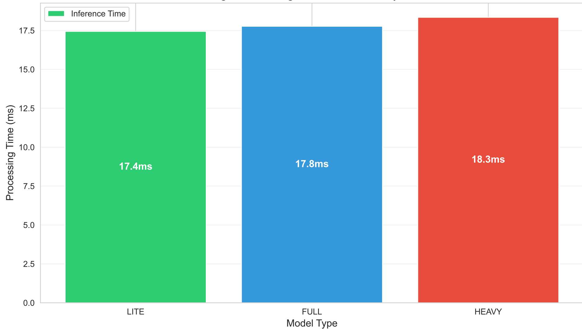
Average Processing Time Breakdown by Model
